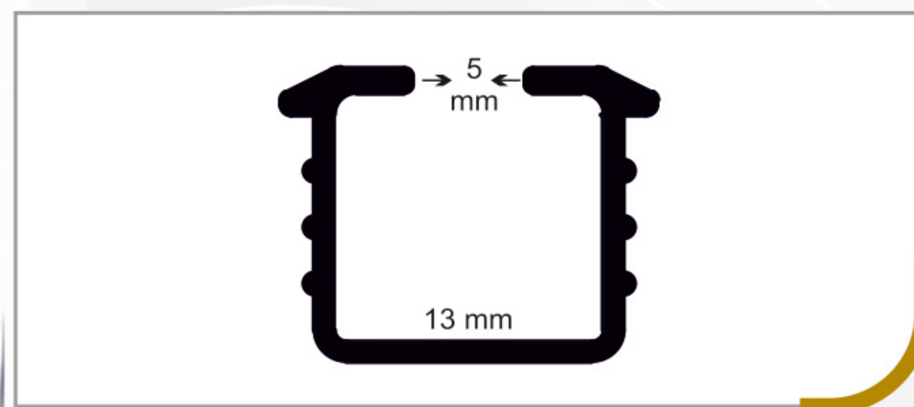
Aluminium Sliding Track
