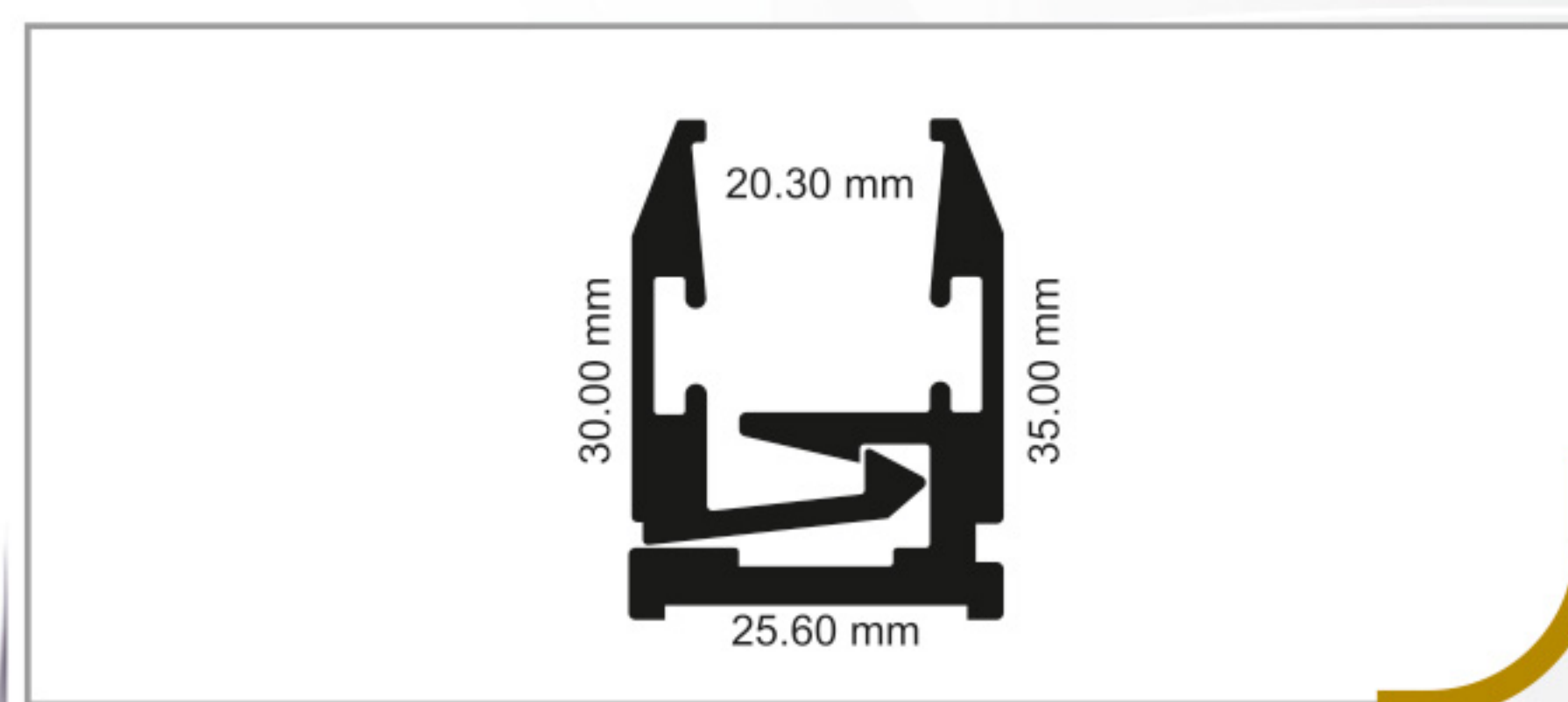
Inter Locking Glazing Profile
