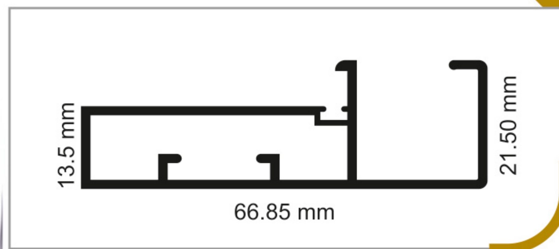
Aluminium Handle Profile (67mm)
