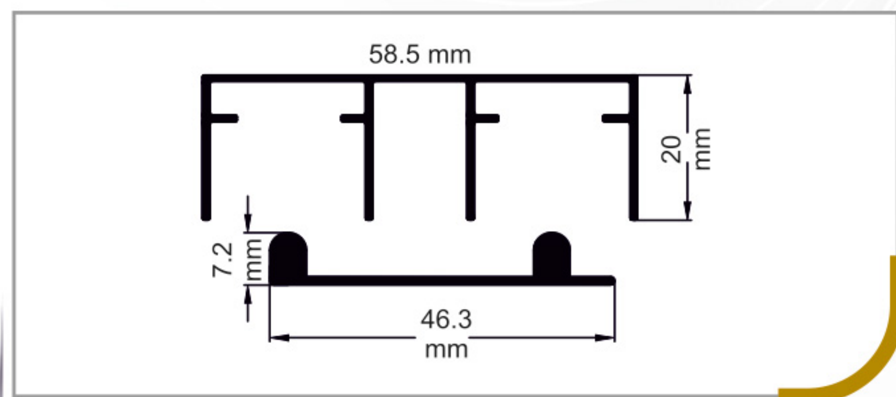
Aluminium Sliding Double Track
