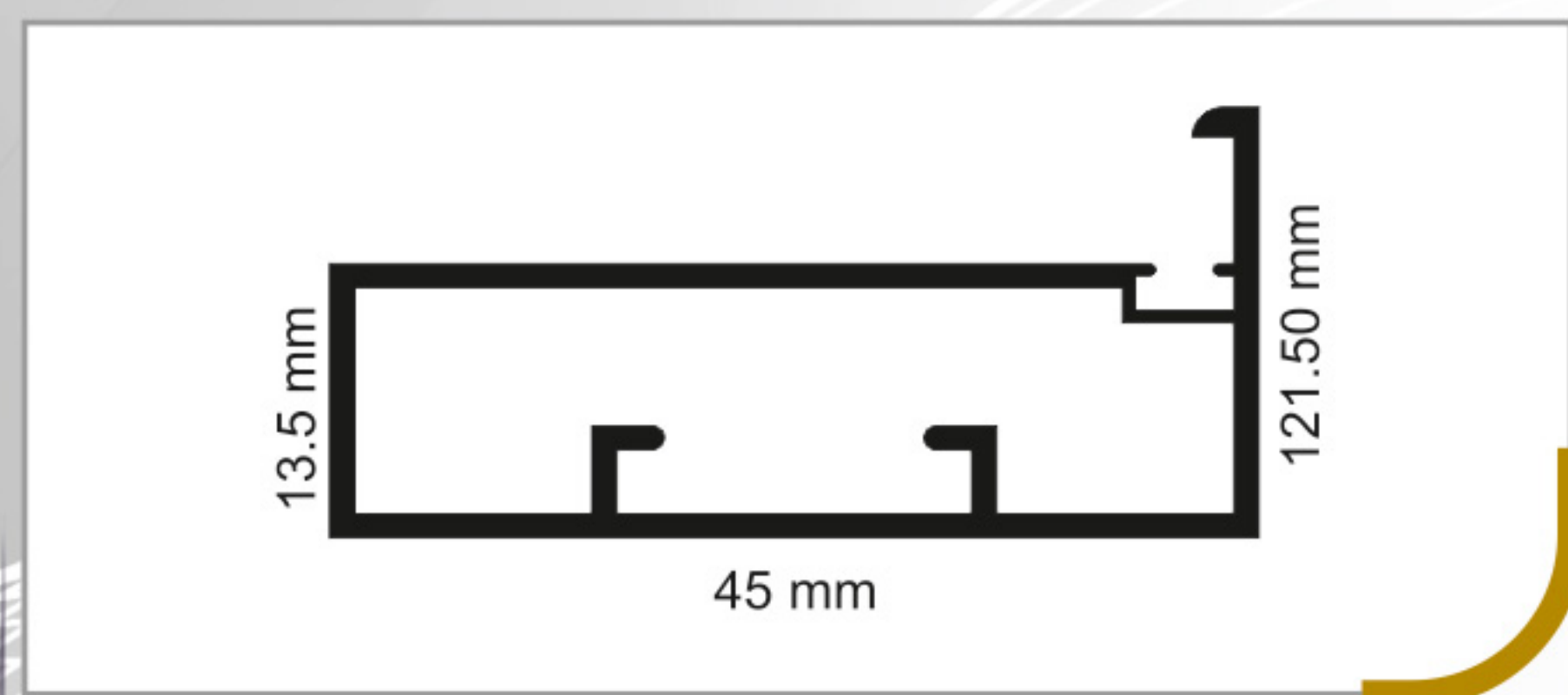
Aluminium Shutter Profile (45mm)
